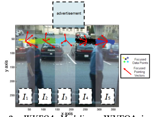
Figure 3: WVFOA Modeling. WVFOA is determined by head pose and horizontal position in the image. The horizontal axis is divided into 5 regions. Yellow, green, cyan, black, and blue data points represent focused training head locations in each region. At the center of each region red arrows represent 4 focused pointing vectors samples.
